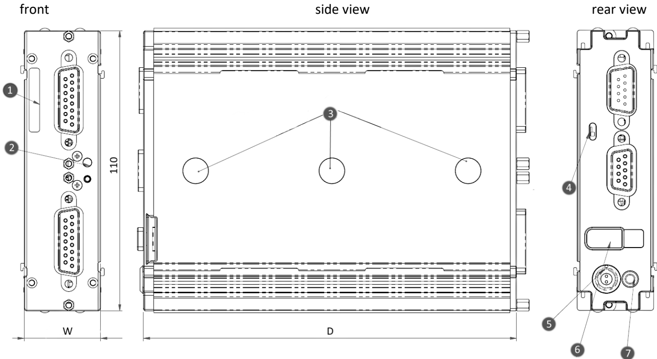
CANFX-module shown in standard operating orientation: housing type L0; width (W) = 30 mm.
